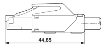
straight plug RJ45 / IP20
