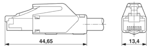
straight plug RJ45 / IP20
